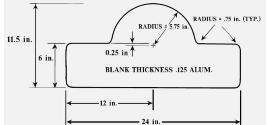
Sign Dimensions
