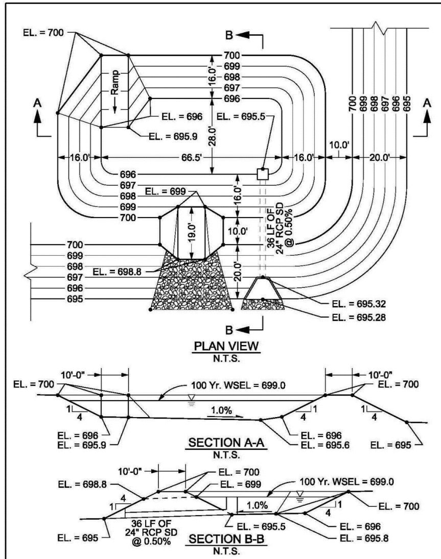
Figure 4.1243 Simple Detention Basin Plan Schematic
