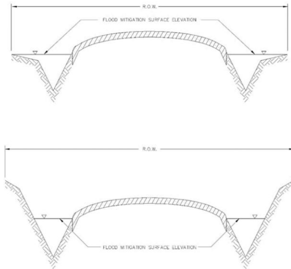
Figure 4.1 Water Spread Limits for Non-Curbed Roadways
