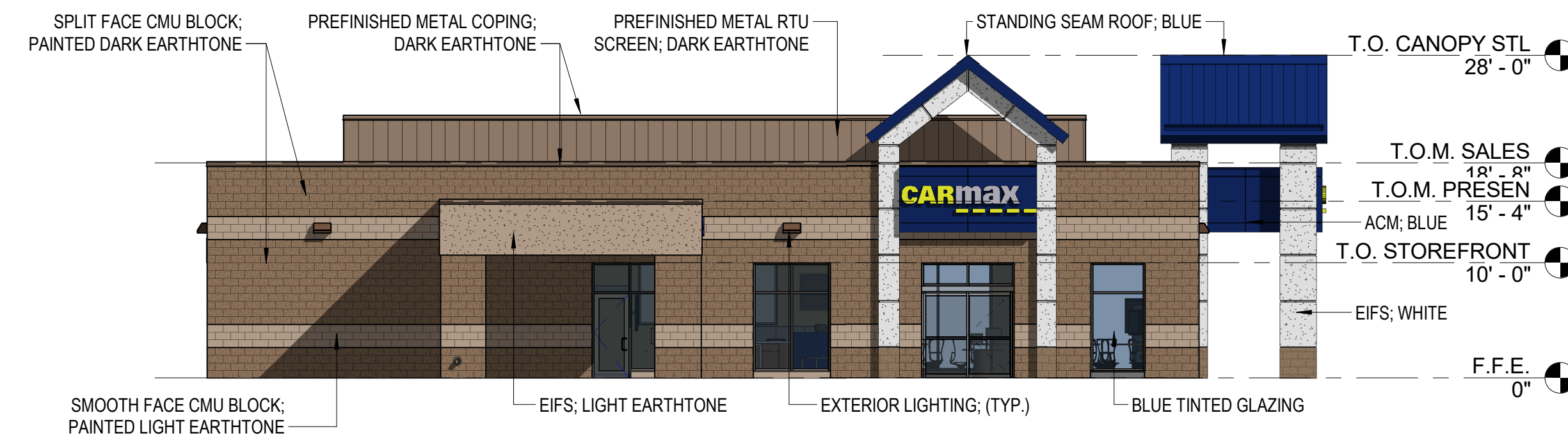
1 EAST A 3.0 3/32" = 1'-0"
