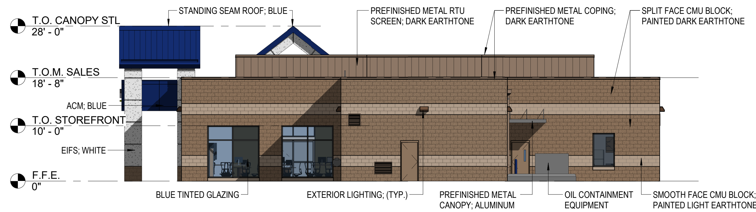
4 WEST A 3.0 3/32" = 1'-0"
