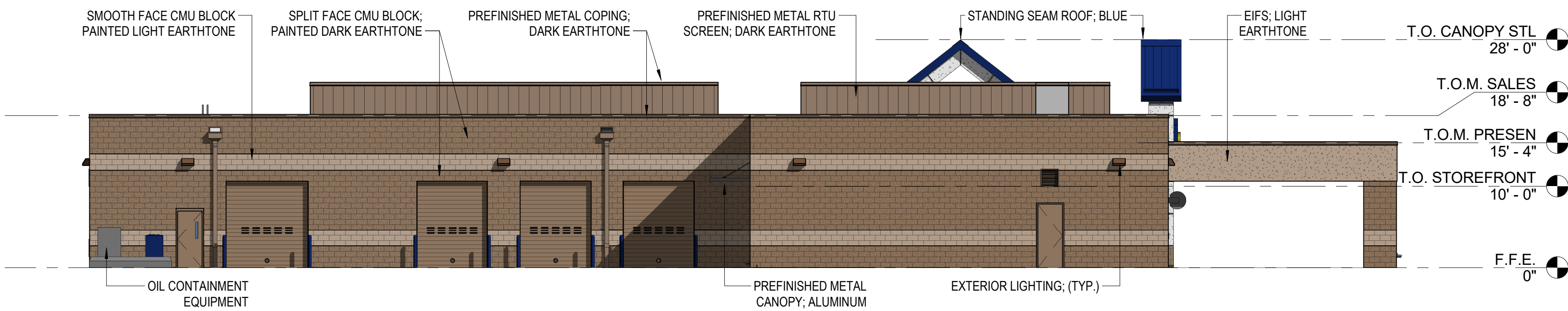
3 SOUTH A 3.0 3/32" = 1'-0"
