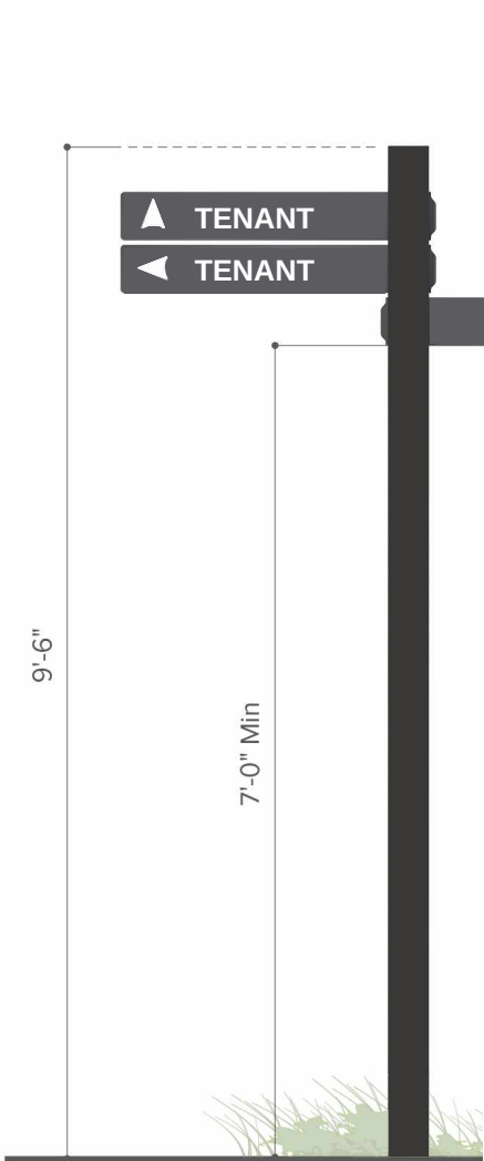
1 Front View Pedestrian Directional
