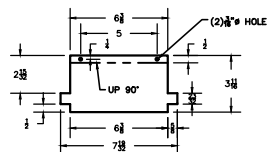
SOCKET LID END CLOSURE
