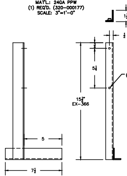
'S'-BOX MNTG. SUPPORT
