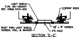
SECTION 'E-E'
