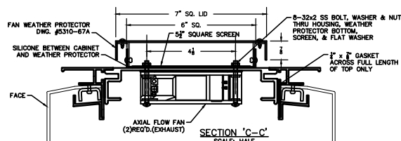
SECTION 'C-C'
