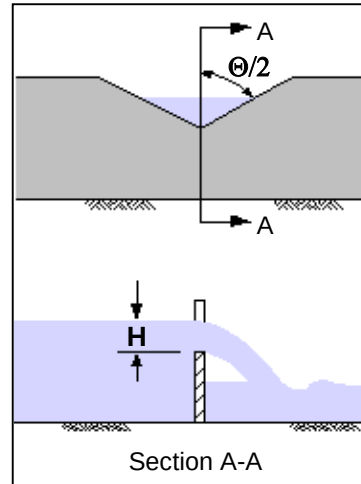
Figure 2.13 V-Notch Weir
