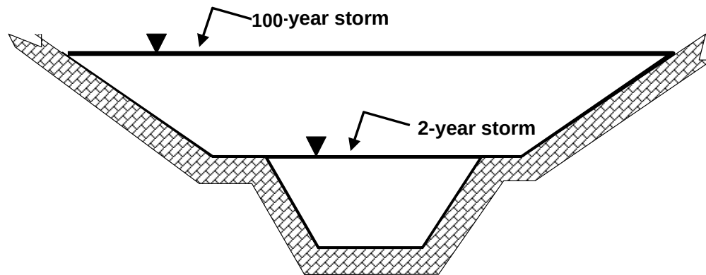
Figure 3.1 Compound Channel
