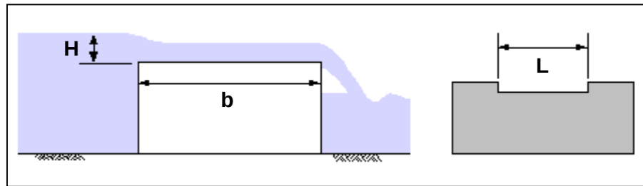
Figure 2.12 Broad-Crested Weir
