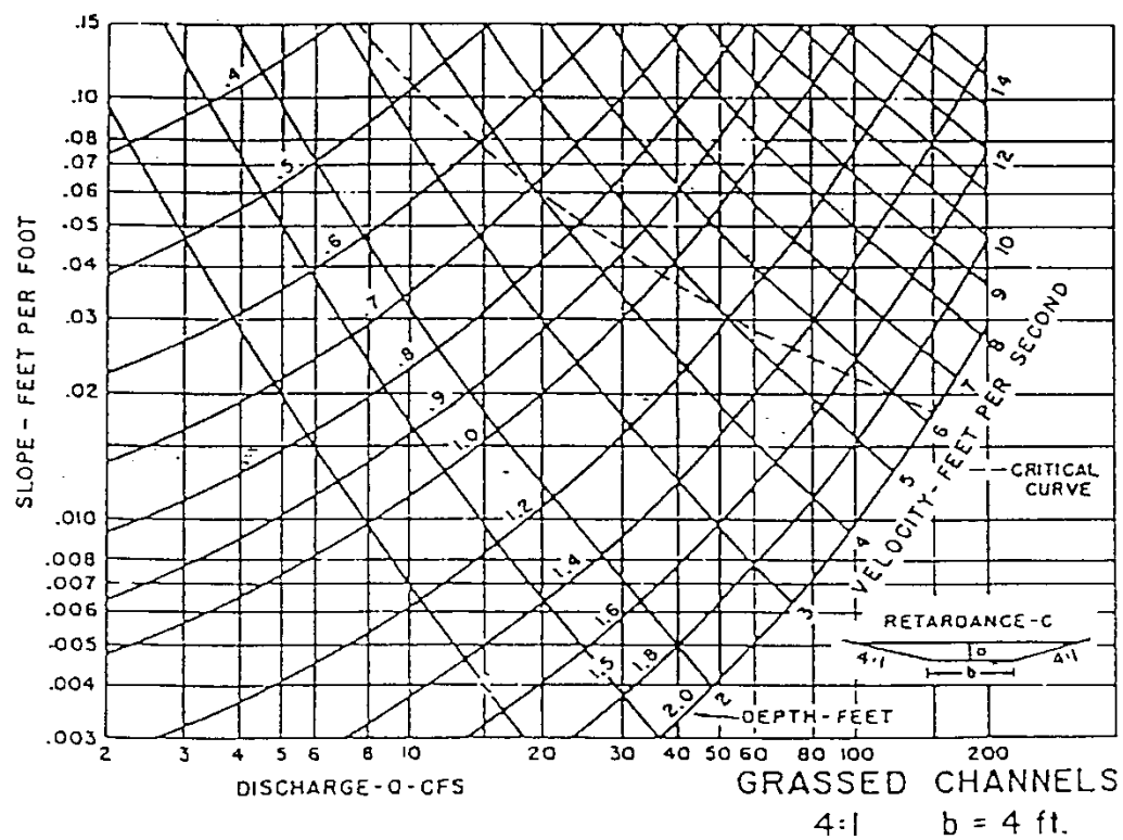
Figure 3.29 Example Nomograph #5
