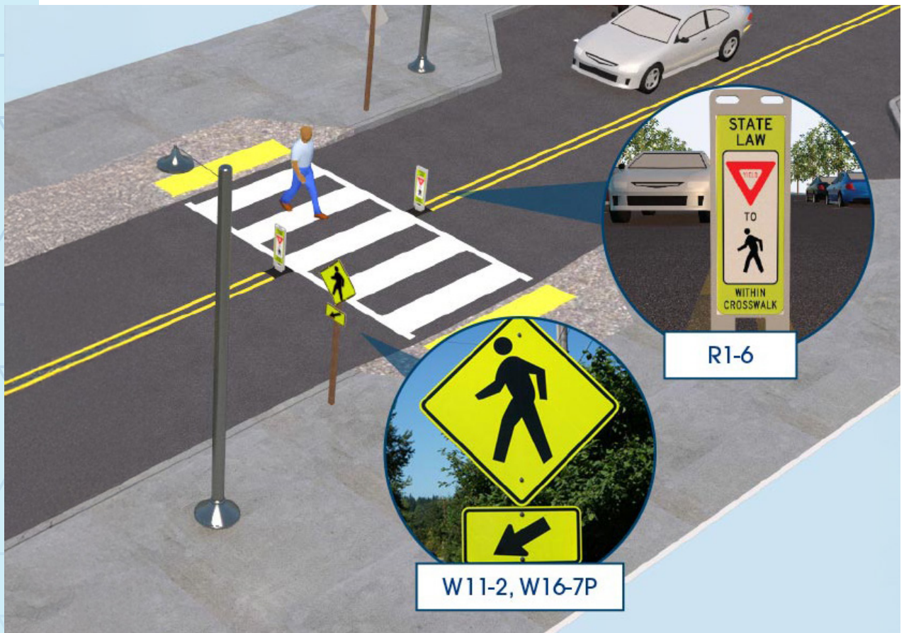
Figure 4.9. Improving Signing and Visibility at Signals Example
