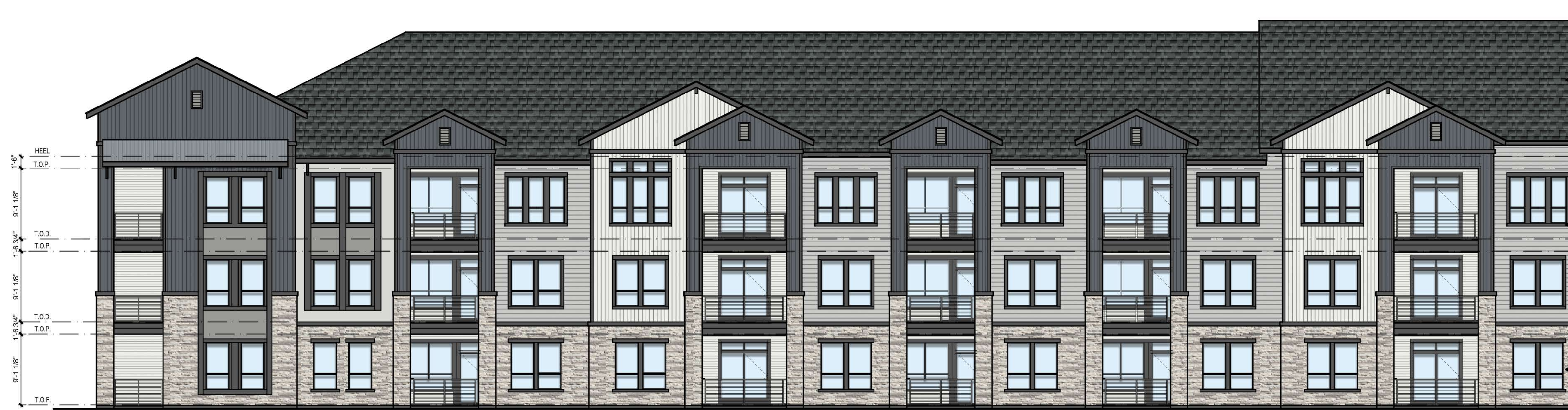
3a BUILDING B - REAR ELEVATION - PART A SCALE: 1" = 1/8"
